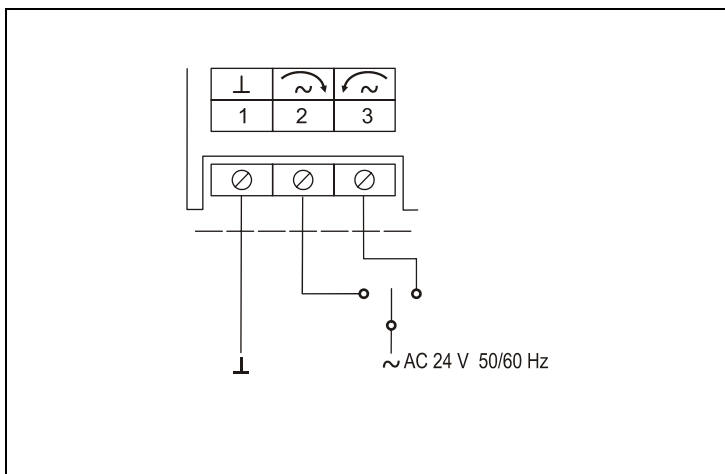
Figure 12: DAB1C and DAD1C Control Wiring Diagram - Floating
