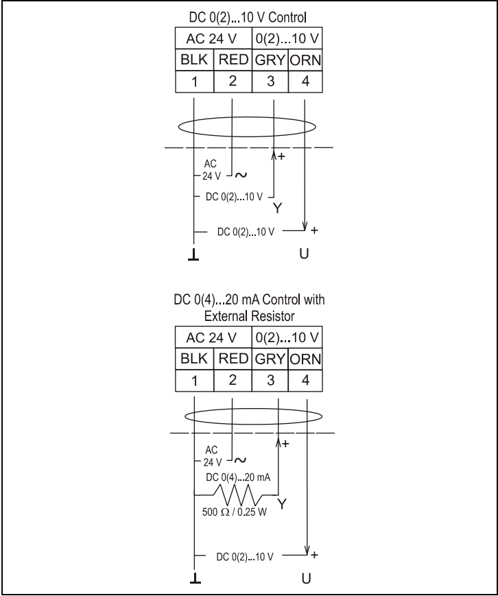
Figure 9: DMD1.2 Control Wiring Diagram
