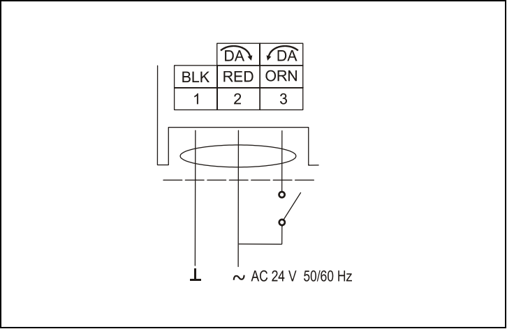
Figure 8: DAB1 and DAD1 Control Wiring Diagram - ON/OFF
